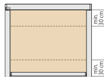
Preferred transverse seam position (option)
