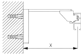
Smart Fix SG 11200 - SG 11205 and bracket SG 3603: Screw (M4x8) needed.
