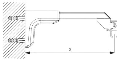
Universal Smart Fix SG 11154 - SG 11156 and bracket SG 3603: Screw (M4x12) needed.
