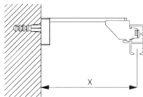
Square Smart Fix SG 11210 - SG 11215 and bracket SG 3603: Screw (M4x8) needed.
