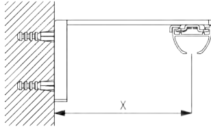
Smart Fix SG 11200 - SG 11205 and clamp SG 3825: Screw (M4x8) needed.
