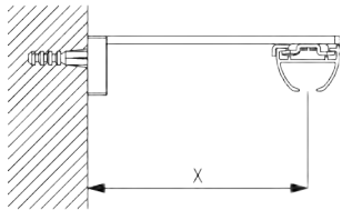
Square Smart Fix SG 11210 - SG 11215 and clamp SG 3825: Screw (M4x8) needed.
