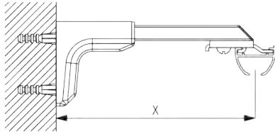
Universal Smart Fix SG 11154 - SG 11156 and bracket SG 3832: Screw (M4x10) needed.
