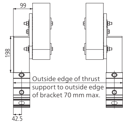
Rafter mounting
