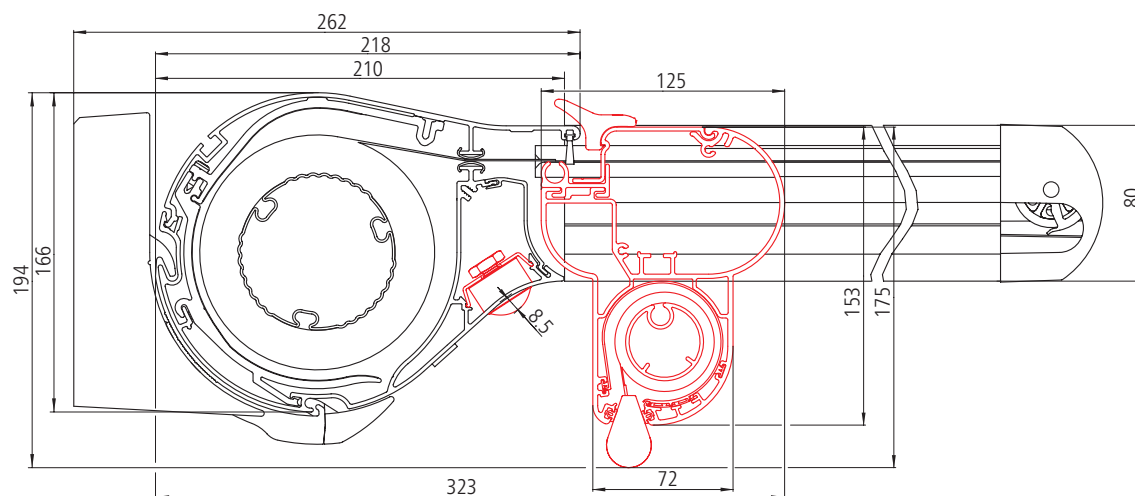
Plaza Viva with wall connection roof cross sections and dimensions
