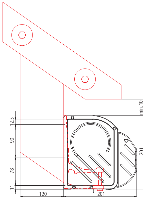
Rafter bracket with mounting plate
