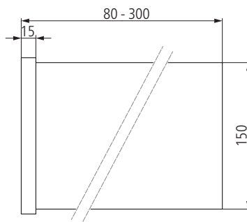
Stand off bracket with wall bracket 180 mm
